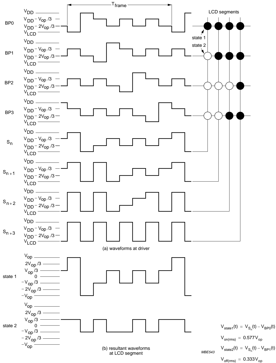
Fig.8 Waveforms for the 1 : 4 multiplex drive mode ( V_{\text{op}} = V_{\text{DD}} - V_{\text{LCD}} ).
